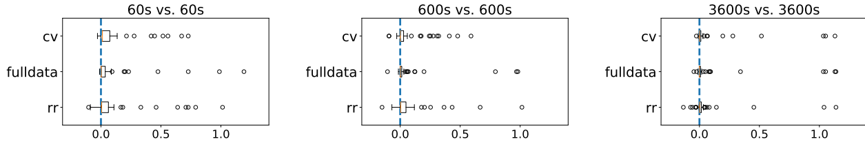
Figure 8. Score difference for FLAML vs. its own alternatives.
