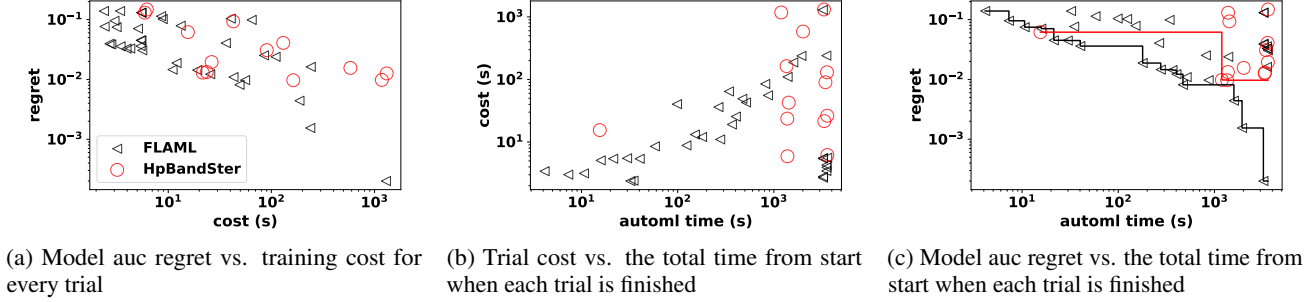
Figure 1. Example of search performance for FLAML vs. a baseline in the same search space. Each marker corresponds to one trial of configuration evaluation in a particular method. Model auc regret=best_auc_model_auc. Each marker corresponds to one trial of configuration evaluation in a particular method. Subfigure (a) suggests that FLAML makes fewer expensive trials with high error (top right corner) than HpBandSter. Subfigure (b) further displays that the expense of trials made by FLAML grows gradually with total time spent, while for HpBandSter there is no such trend. As a result, subfigure (c) shows that FLAML outperforms in both early and late stages.
